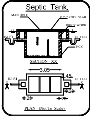
Septic Tank.
