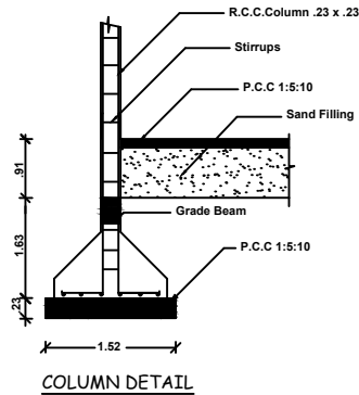
COLUMN DETAIL
