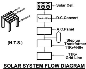
SOLAR SYSTEM FLOW DIAGRAM
