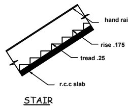
STAIR
