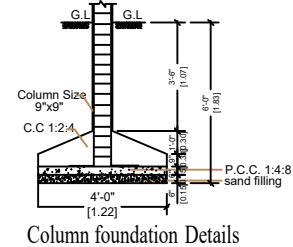
Column foundation Details
