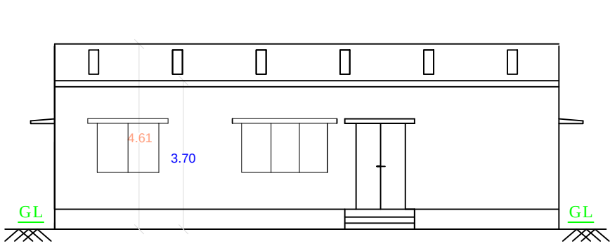
FRONT ELEVATION
