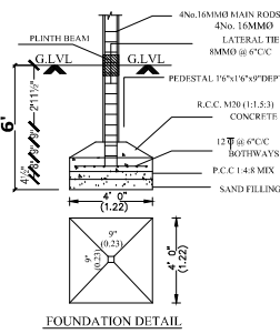
FOUNDATION DETAIL
