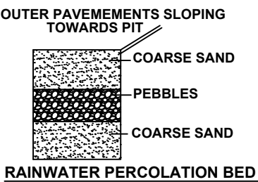
RAINWATER PERCOLATION BED
