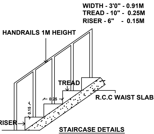
STAIRCASE DETAILS
