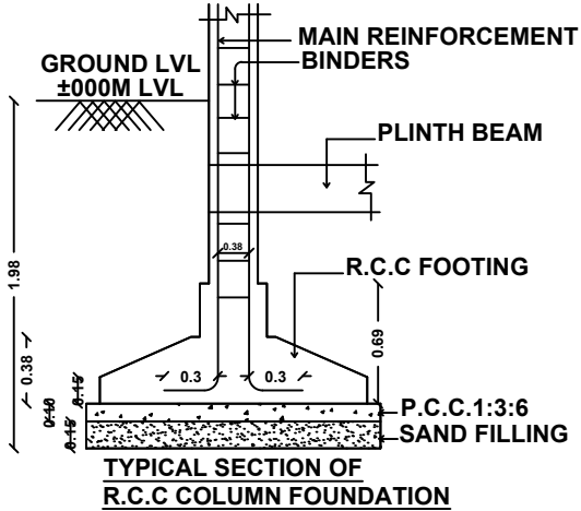
TYPICAL SECTION OF R.C.C COLUMN FOUNDATION
