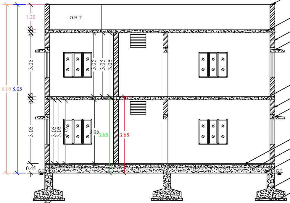
SECTION-AB
