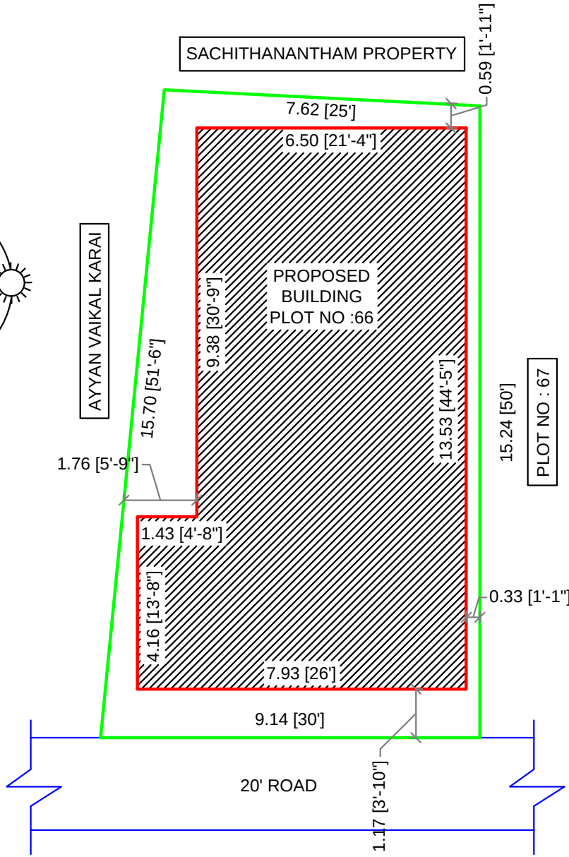
SITE PLAN (1:100)
