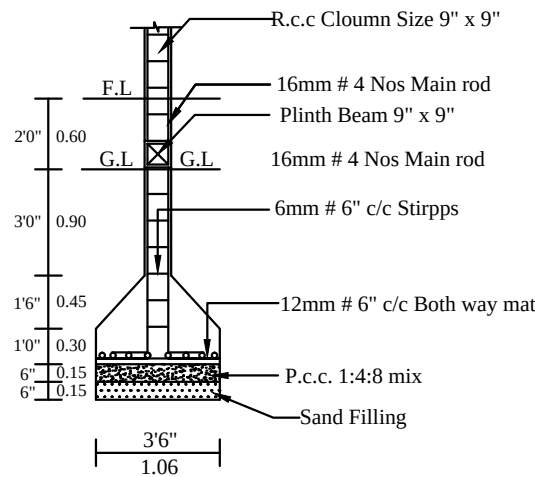
COLUMN DETIAL
