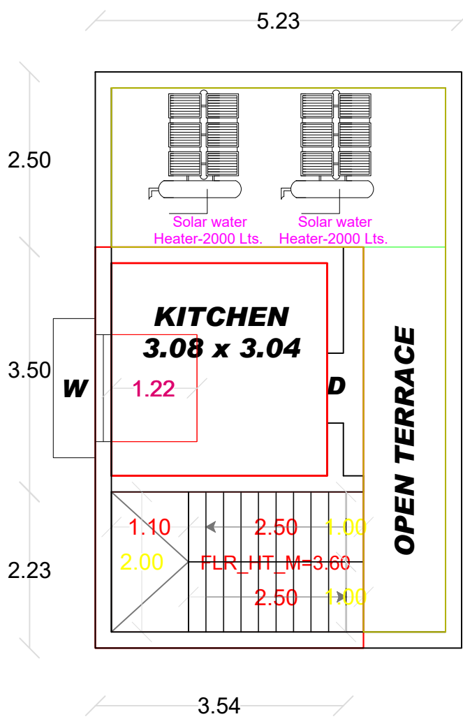
FIRST FLOOR PLAN OPEN TERRACE PLAN
