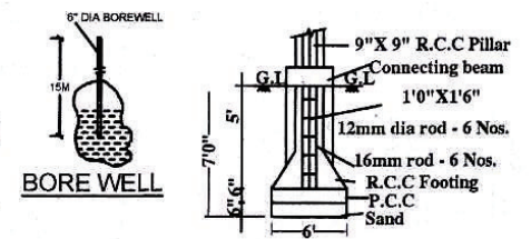
FOUNDATION DETAILS
