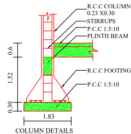
COLUMN DETAILS
