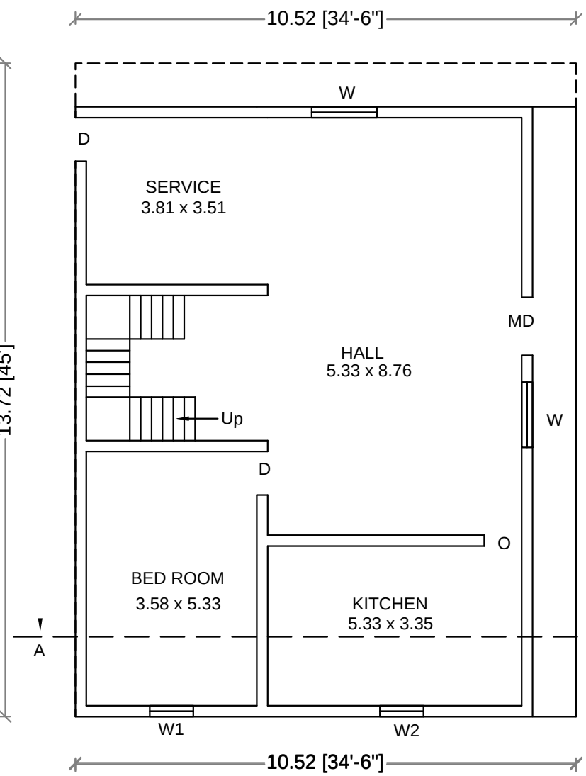
R PLAN
