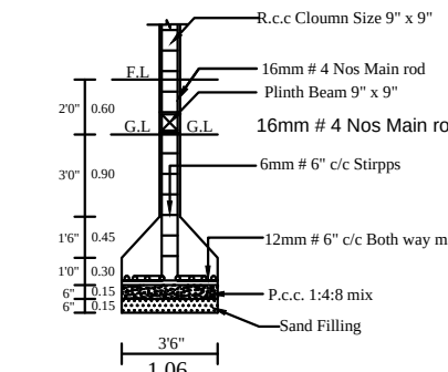
COLUMN DETIAL
