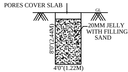
RAINWATER HARVESTING UNIT
