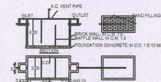
SEPTIC TANK & DISPERSION TRENCH
