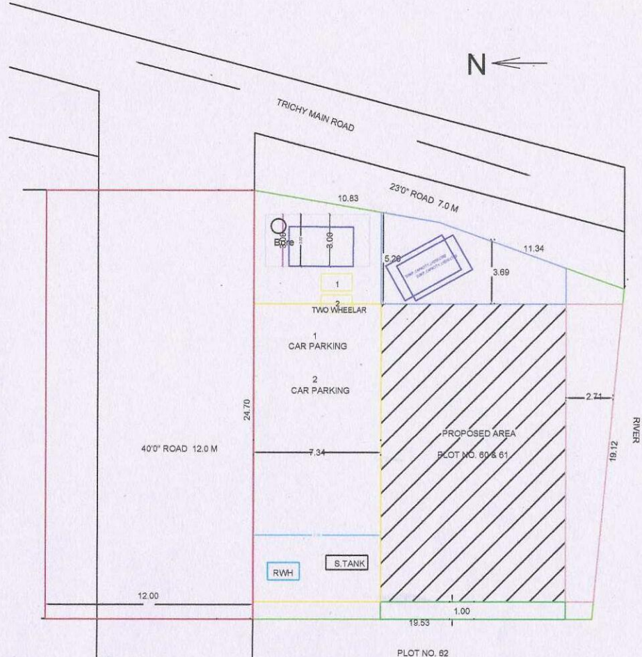
SITE PLAN 1: 100
