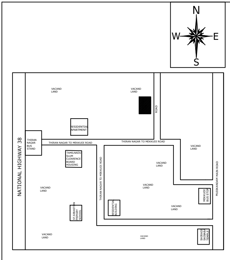
KEY PLAN
