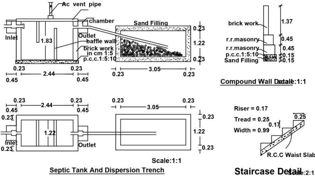
Septic Tank And Dispersion Trench
