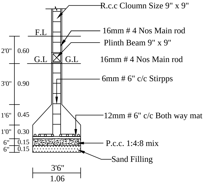
COLUMN DETIALS
