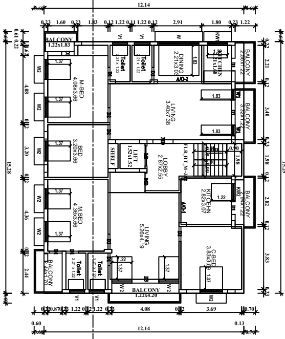
TYPICAL_FLOOR_PLAN=1,2,3, (FIRST, SECOND & THIRD FLOOR)
