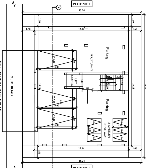
SILT FLOOR CUM SITE PLAN
