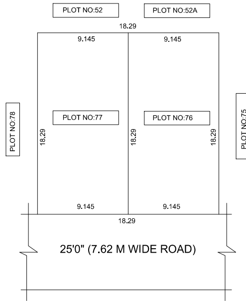
AMALGAMATION OF PLOTS 76 & 77
