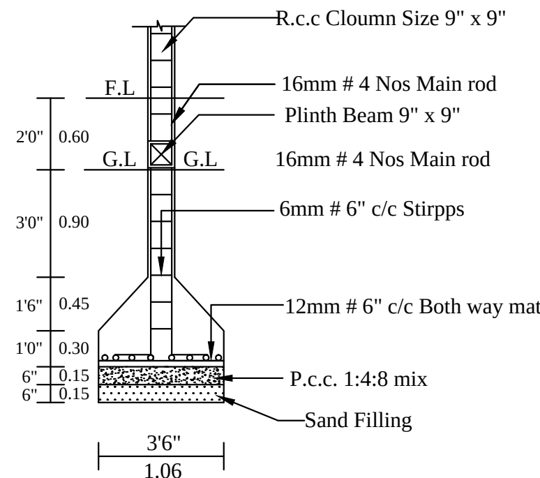
COLUMN DETAILS
