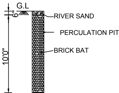
PERCULATION PIT
