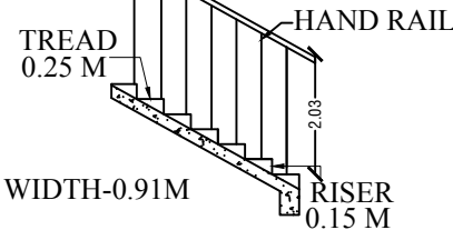
STAIRCASE DETAILS
