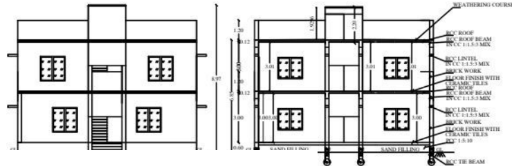
SECTION AB
