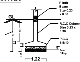
FOUNDATION DETAILS
