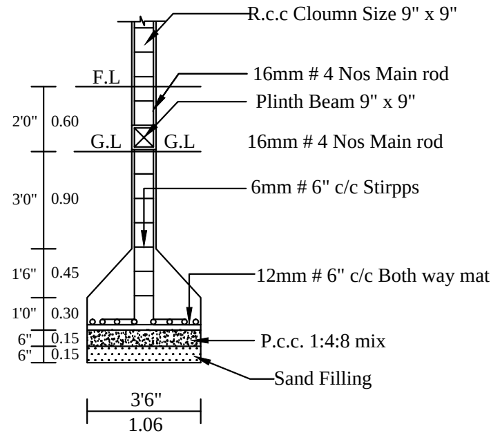
COLUMN DETAILS
