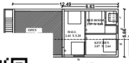
ST FLOOR PLAN
