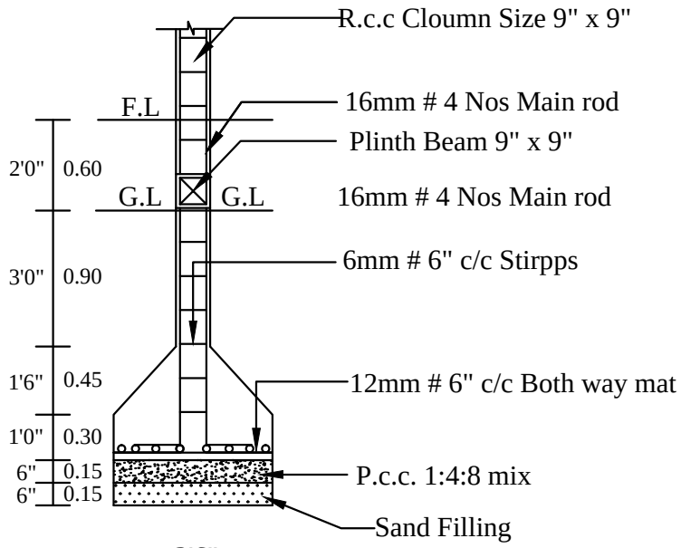
COLUMN DETIALS
