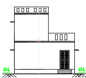
FRONT ELEVATION
