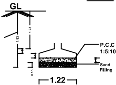
FOUNDATION DETAILS
