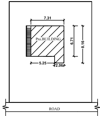
SITE PLAN
