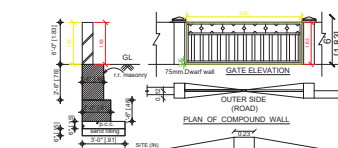
COMPOUND WALL DETAIL SECTION ON DWARF WALL
