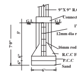
FOUNDATION DETAILS
