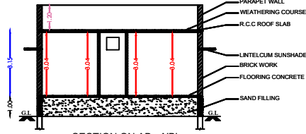
SECTION ON AB, A'B' BLOCK1, BLOCK2
