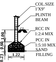
COLUMN DETAILS
