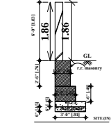
COMPOUND WALL
