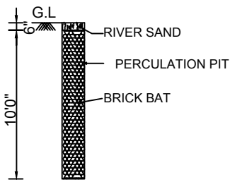
PERCOLATION PIT
