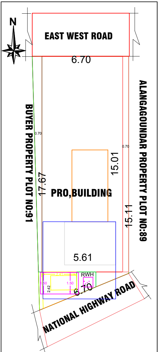
SITE PLAN
