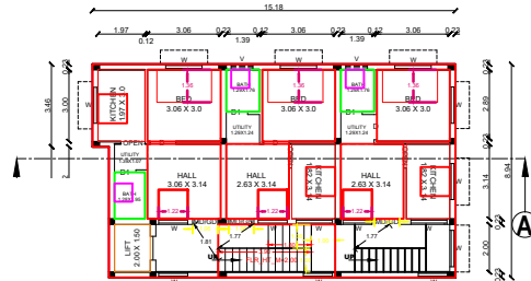
PROPOSED FIRST FLOOR PLAN
