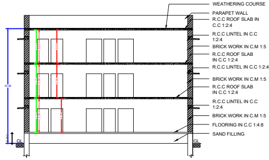
SECTION ON-AA
