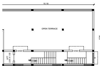
PROPOSED OPEN TERRACE FLOOR PLAN
