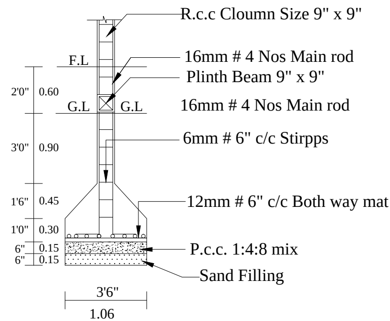
COLUMN DETIAL
