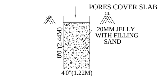
RAIN WATER HARVESTING UNIT
