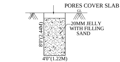
RAIN WATER HARVESTING UNIT
