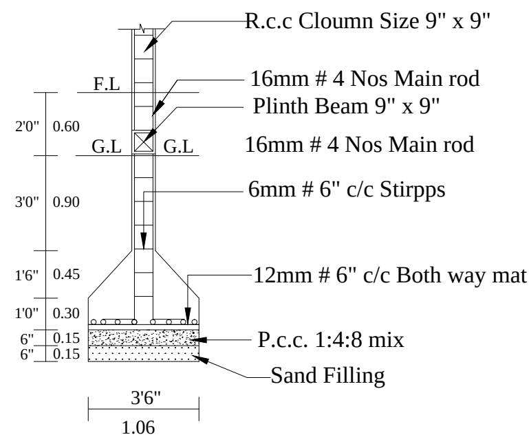
COLUMN DETIAL
