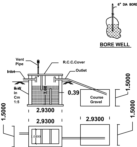
SEPTIC TANK & D-TRENCH DETAILS
