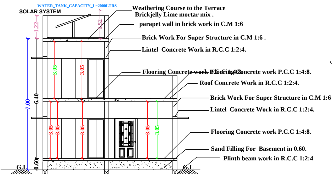
SECTION-AB
