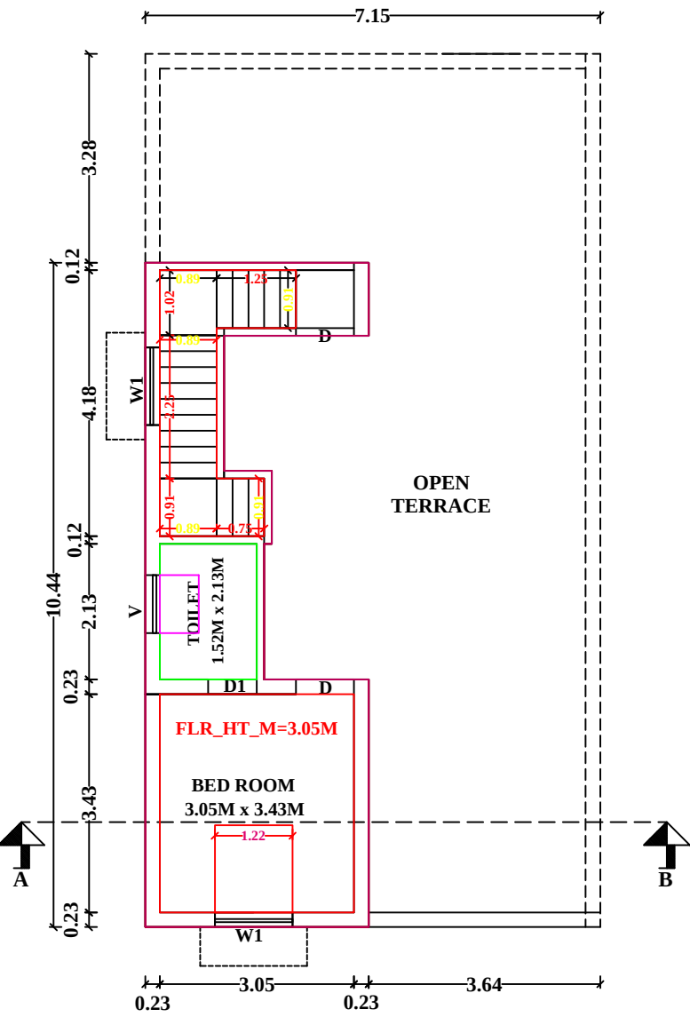
FLOOR-1 PRO-FIRST FLOOR PLAN
