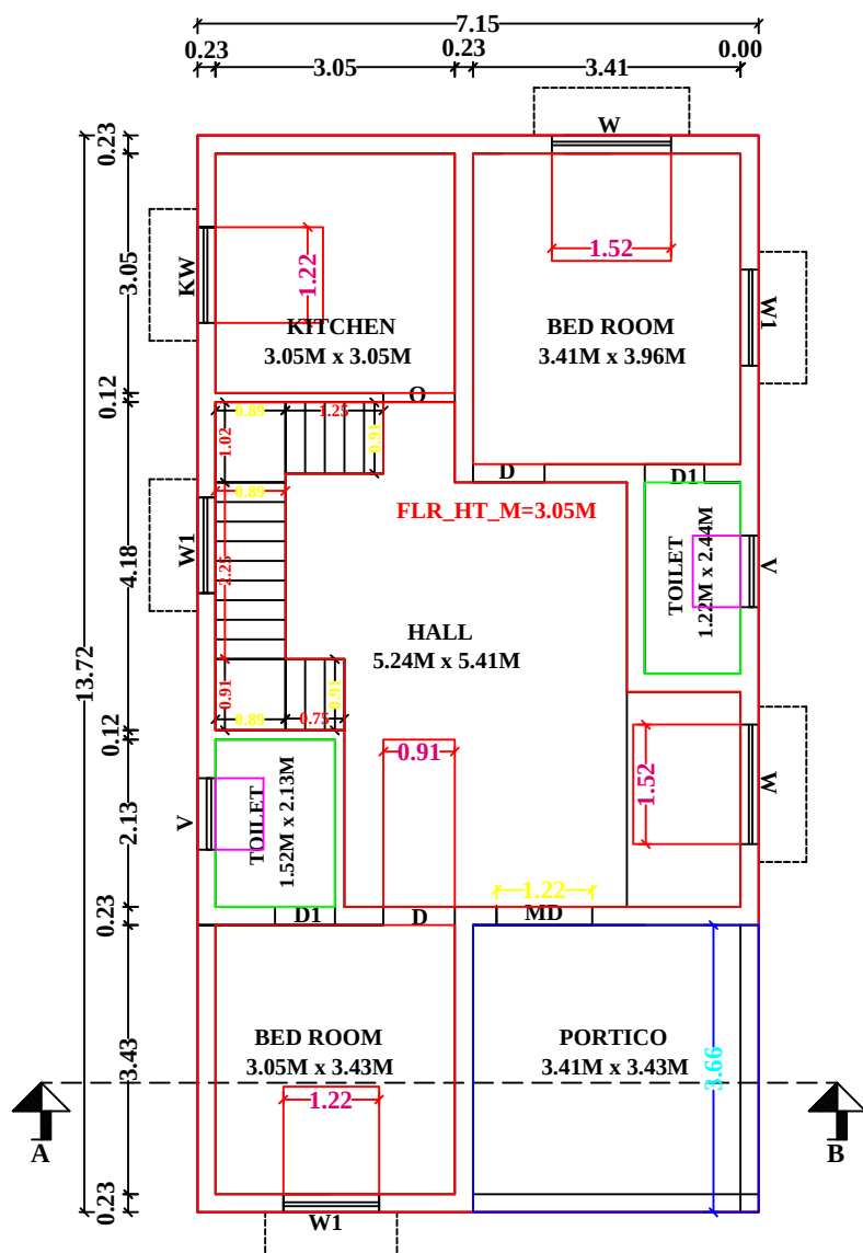
FLOOR-0
