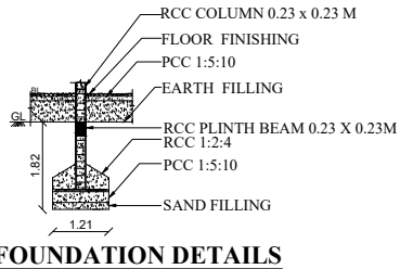
FOUNDATION DETAILS
