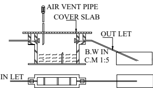
DETAILS OF SEPTIC TANK & D-TRENCH
