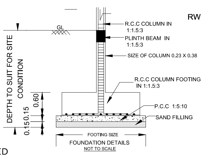
FOUNDATION DETAILS NOT TO SCALE
