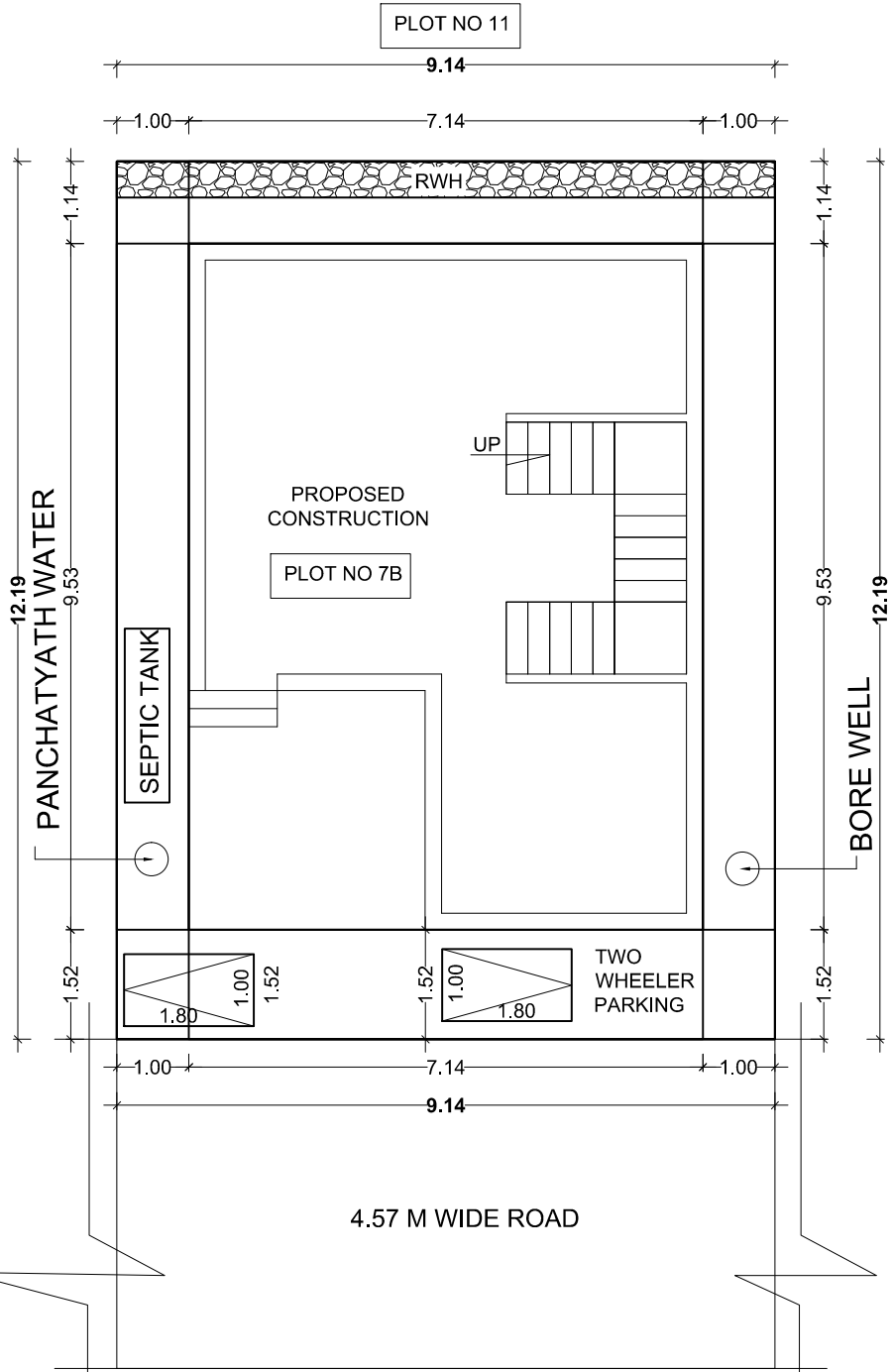
SITE PLAN
