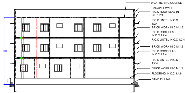
SECTION ON-AA
