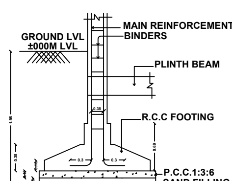
TYPICAL SECTION OF R.C.C COLUMN FOUNDATION
