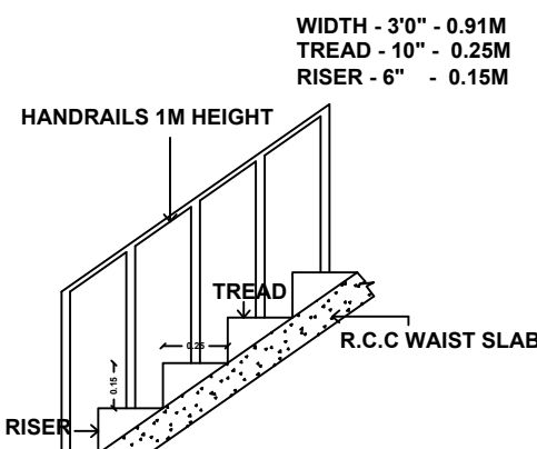
STAIRCASE DETAILS
