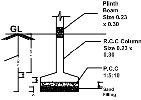
FOUNDATION DETAILS
