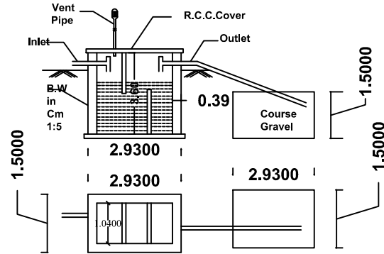
SEPTIC TANK & D-TRENCH DETAILS
