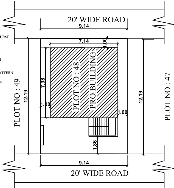
SITE PLAN
