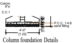
Column foundation Details
