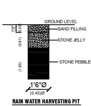
RAIN WATER HARVESTING PIT
