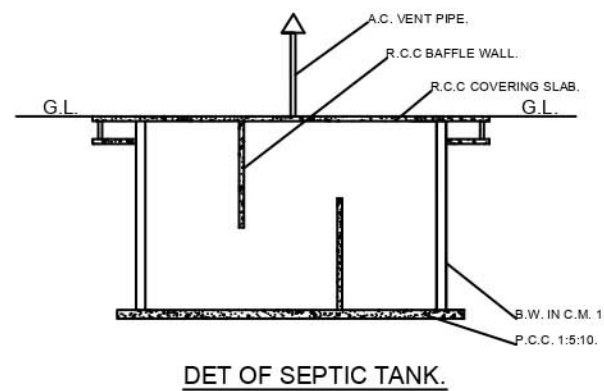
DET OF SEPTIC TANK.
