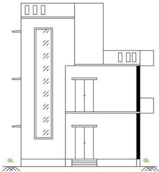
FRONT ELEVATION
