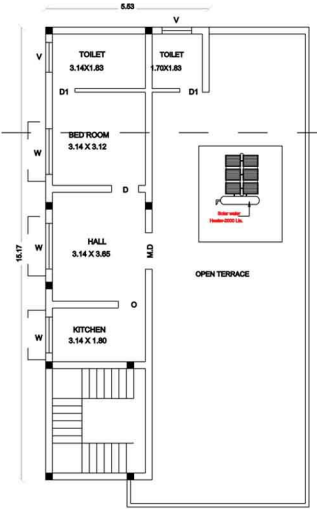
PRO.SECOND FLOOR PLAN
