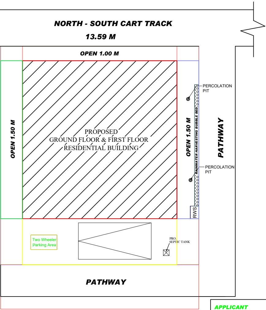
SITE PLAN (SCALE 1:1)
