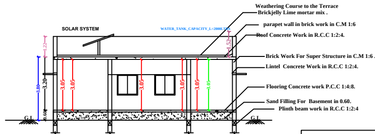
SECTION-AB
