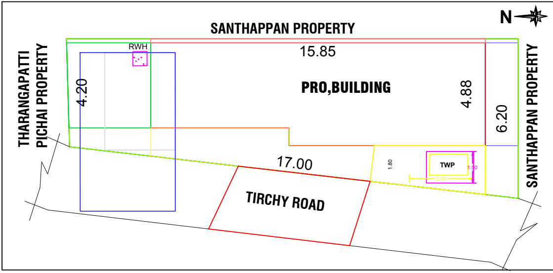
SITE PLAN
