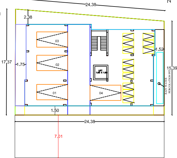
SITE PLAN
