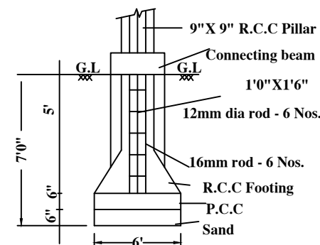
COLOUMN FOUNDATION DETAILS
