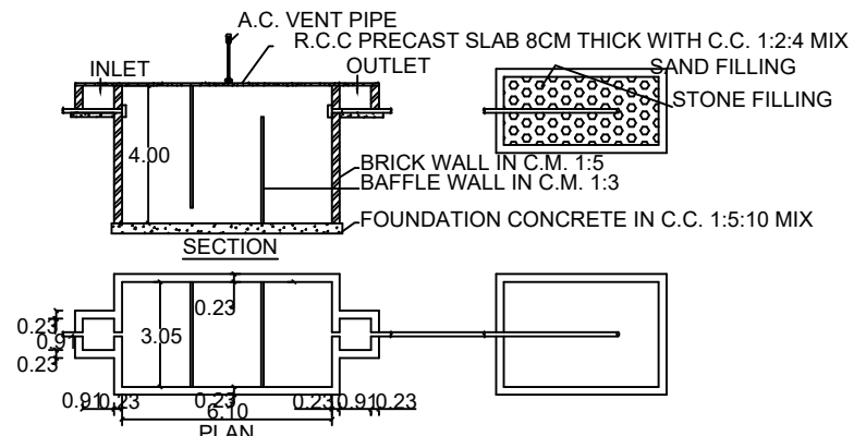
PLAN & SECTION OF SEPTIC TANK & DISPERSION TRENCH
