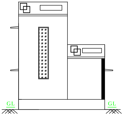
FRONT ELEVATION
