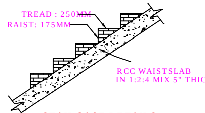
STAIRCASE DETAILS
