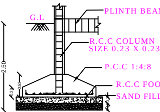
TYPICAL SECTION OF R.C.C COLOUMN FOOTING
